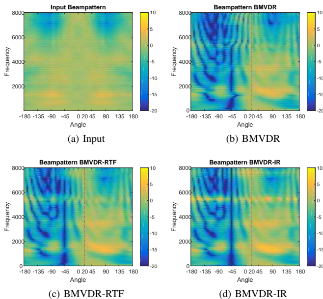
Fig. 3: Beampattern of the BMVDR, BMVDR-RTF and BMVDR-IR ( \eta = 0 ) beamformers, together with the input beampattern (anechoic environment, desired source at 20^\circ , interfering source at -45^\circ , M = 3 ).
