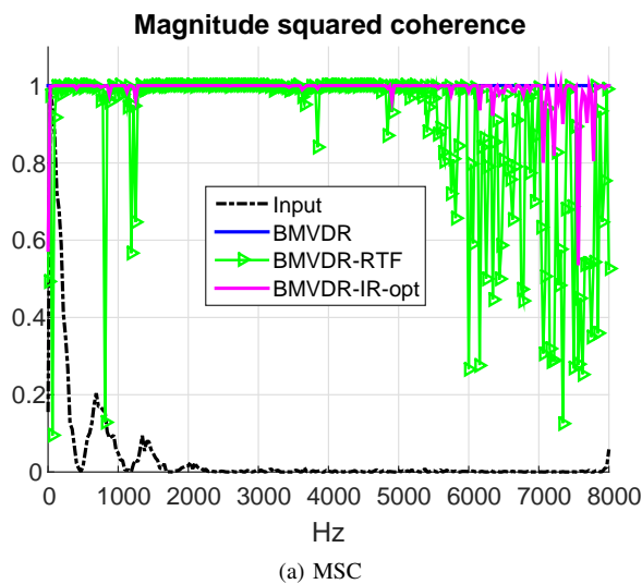
Fig. 6: The MSC for diffuse noise field at the input and at the output of the BMVDR, BMVDR-RTF and BMVDR-IR ( \eta = \eta_{opt} ) beamformers (Office, desired source at 20^\circ , interfering source at -45^\circ , M = 3 ).
