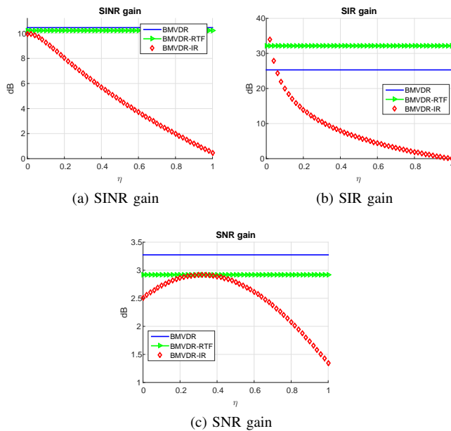
Fig. 5: Global binaural SINR, SIR and SNR gains for BMVDR, BMVDR-RTF and BMVDR-IR beamformers as a function of \eta (Office environment, desired source at 20^\circ , interfering source at -45^\circ , M = 3 ).
